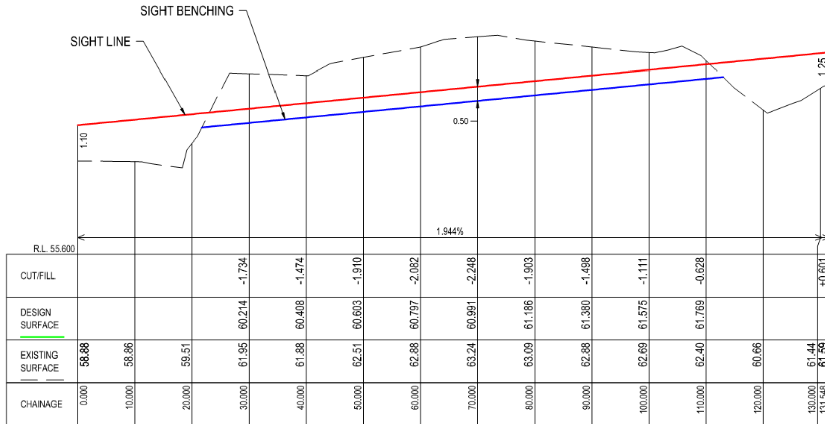
LONGITUDINAL SECTION SISD 'B' Ch 0.000 to Ch 131.548 SCALES: HORIZONTAL 1:500 VERTICAL 1:100
