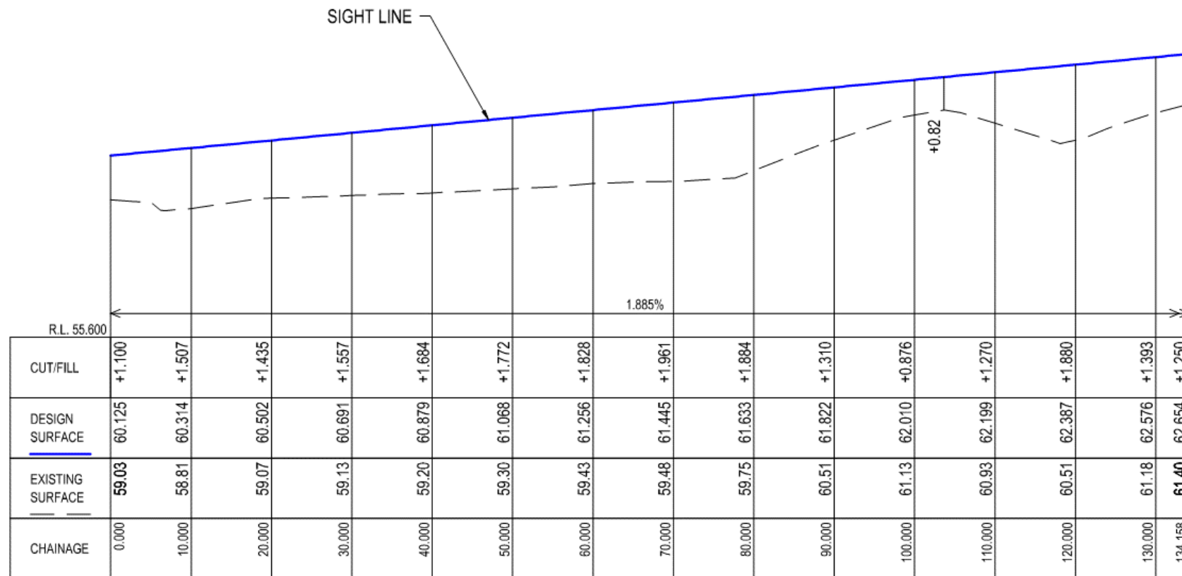
LONGITUDINAL SECTION JUNCTION SISD 'A' Ch 0.000 to Ch 134.158 SCALES: HORIZONTAL 1:500 VERTICAL 1:100
